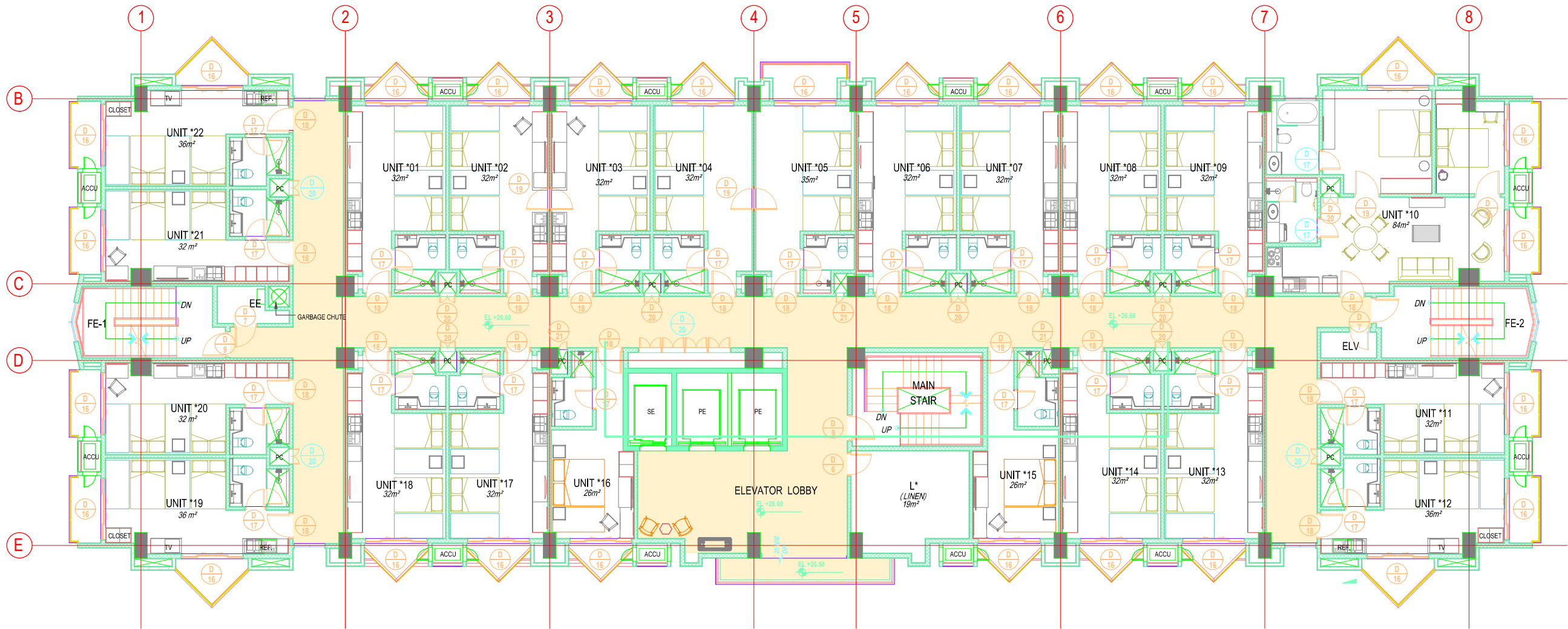
TYPICAL SEVENTH TO EIGHTH FLOOR PLAN
