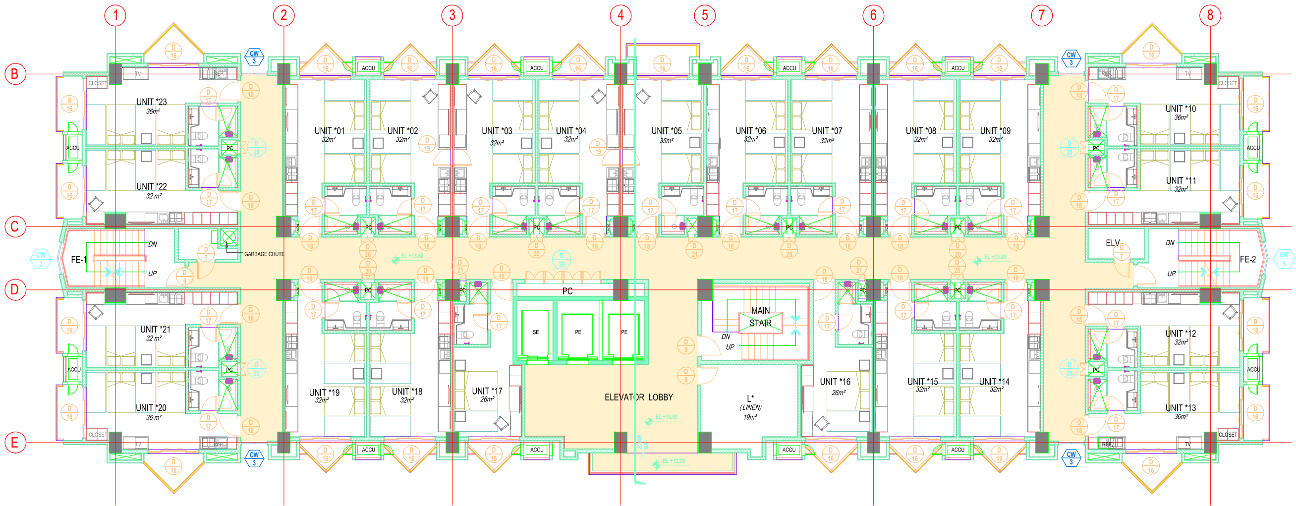
TYPICAL FOURTH TO SIXTH FLOOR PLAN
